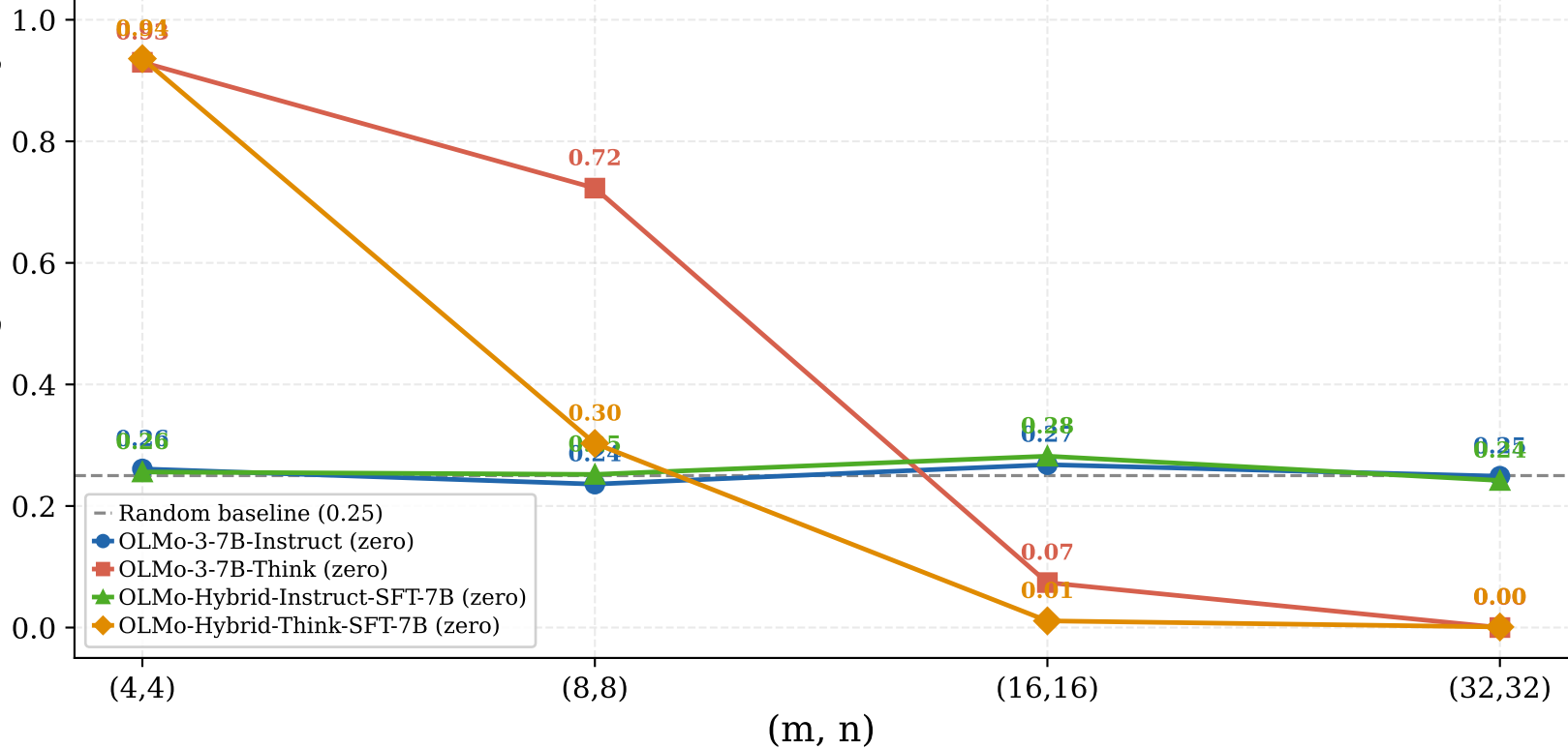
Parsed Weighted Accuracy
